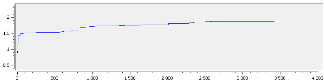
Figure 5: Dependency between generation and fitness F_A .
