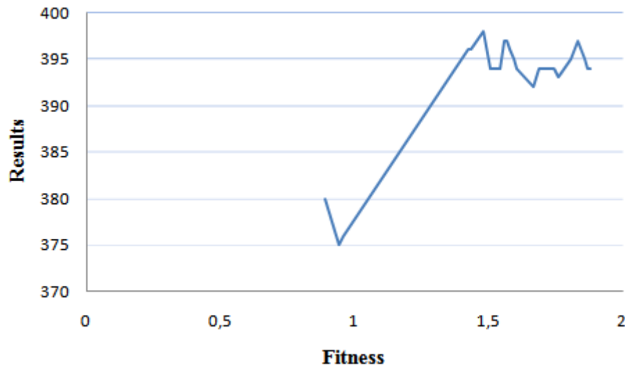
Figure 7: Dependency between fitness F_A and number of correctly recognized samples from testing data (maximum number of recognized samples was 398).
