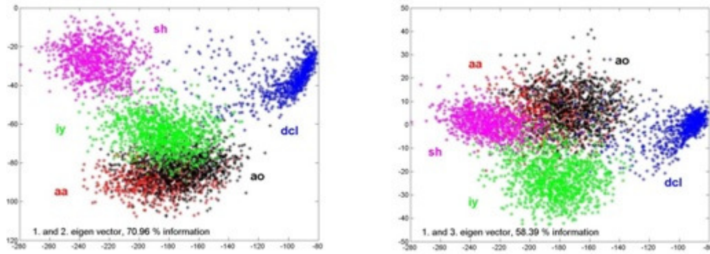
Figure 2: Projection of input data into planes formed by vectors (u_1, u_2) and (u_1, u_3)
