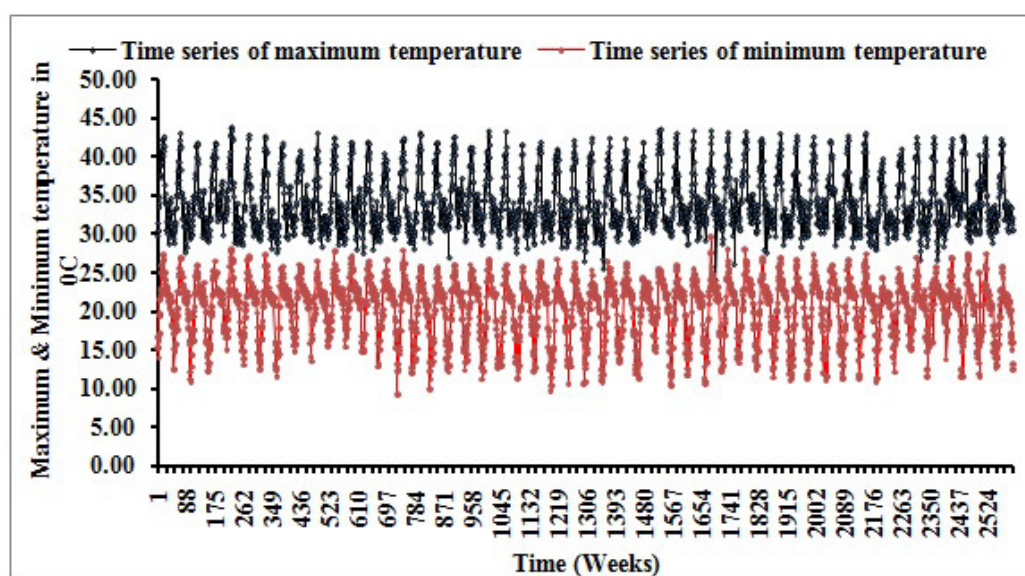
Fig. 1: Weekly maximum and minimum temperature series pertaining to Solapur region from 1969 to 2018
