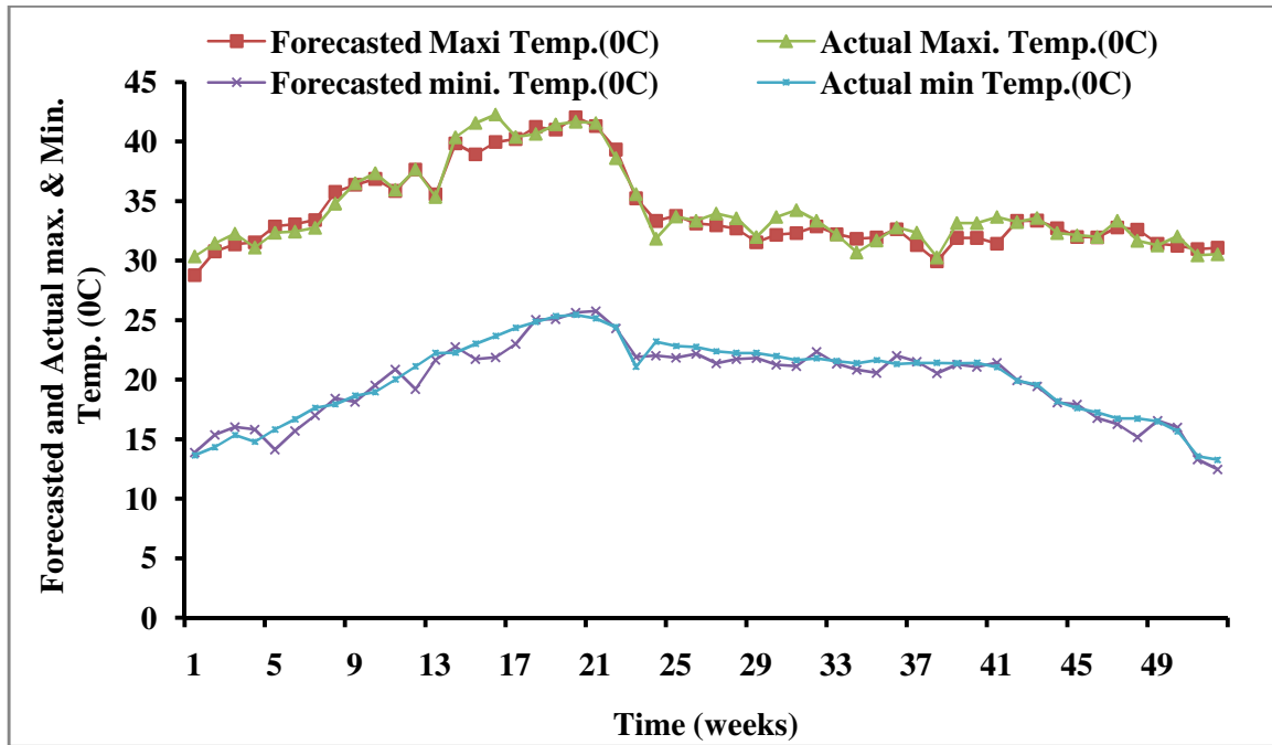
Fig. 6: Comparison of forecasted and actual maximum and minimum temperature in ^{\circ}\text{C} by ARIMA (0,0,1)(1,1,0) 52 and ARIMA (0,0,1)(0,1,1) 52 model.
