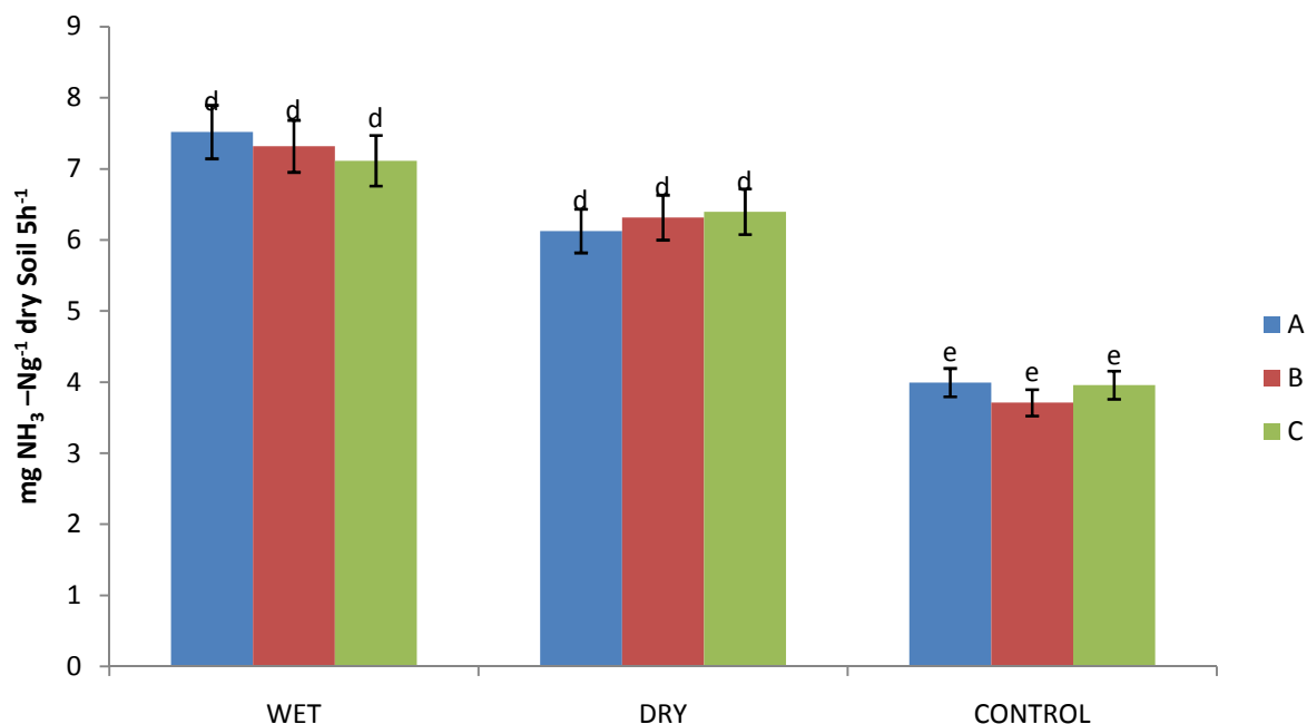
Fig 10: Cassava Mill effluent (CME) infiltrated soil urease activities( \text{mg NH}_3\text{-Ng}^{-1}\text{ dry Soil } 5\text{h}^{-1} ). Wet and dry season.
