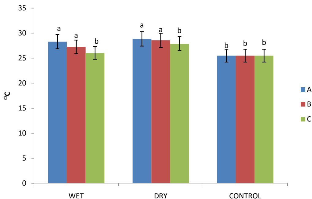
Fig 1 Cassava Mill effluent (CME) infiltrated soil temperature (°C) wet and dry season.
